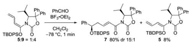
Scheme 4. Reactivity of E - and Z -Enolates
